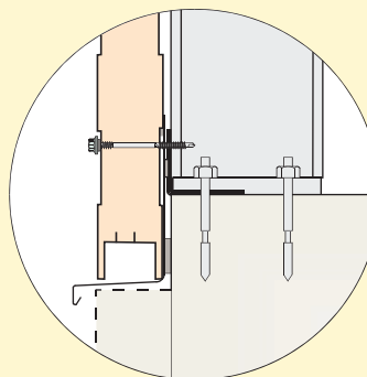
Detail soklu
